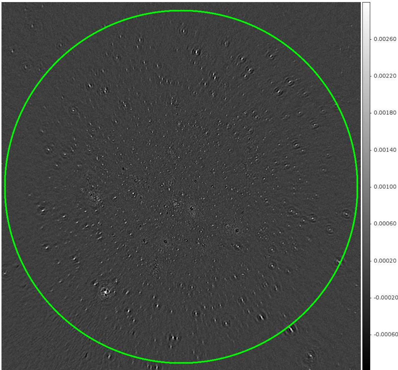
Fig. 9. The NCP image after multi-directional calibration and source subtraction using SAGECal. After a shallow deconvolution using CASA (mainly to estimate the PSF), the skymodel is restored onto the image. The circle indicates an area of diameter 10 degrees. The image has 12000 \times 12000 pixels of size 4'' with a PSF of 12'' and the noise level is about 100\ \mu\text{Jy/PSF} . Due to the fact that RS and CS beam shapes have different FOVs the sources at the edge of the image are distorted. In addition, due to frequency smearing, the sources at the edge of the image appear 'attracted' towards the center. The colourbar units are in Jy/PSF.
